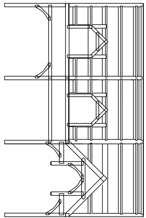
South Frame Elevation Timber framed porch not shown
